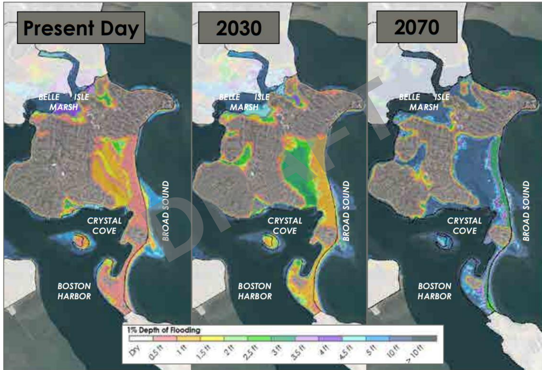
Figure 3-4 Winthrop Depth of Flooding (1% Chance water level)
